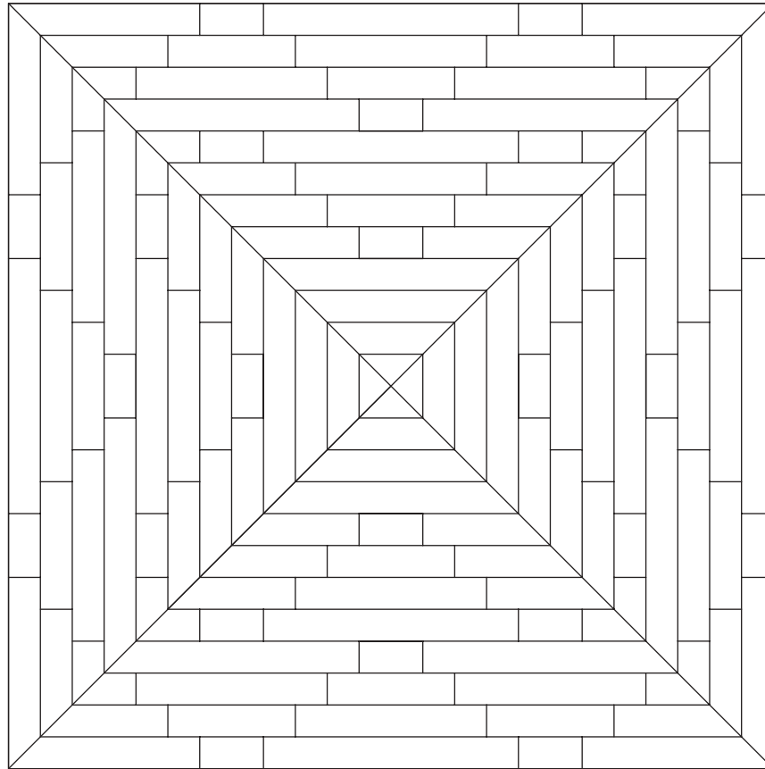
PATTERN #9 6" RANDOM LAYOUT 12' X 12' AREA SHOWN 144 sq. ft. = 29 Units of Planking
