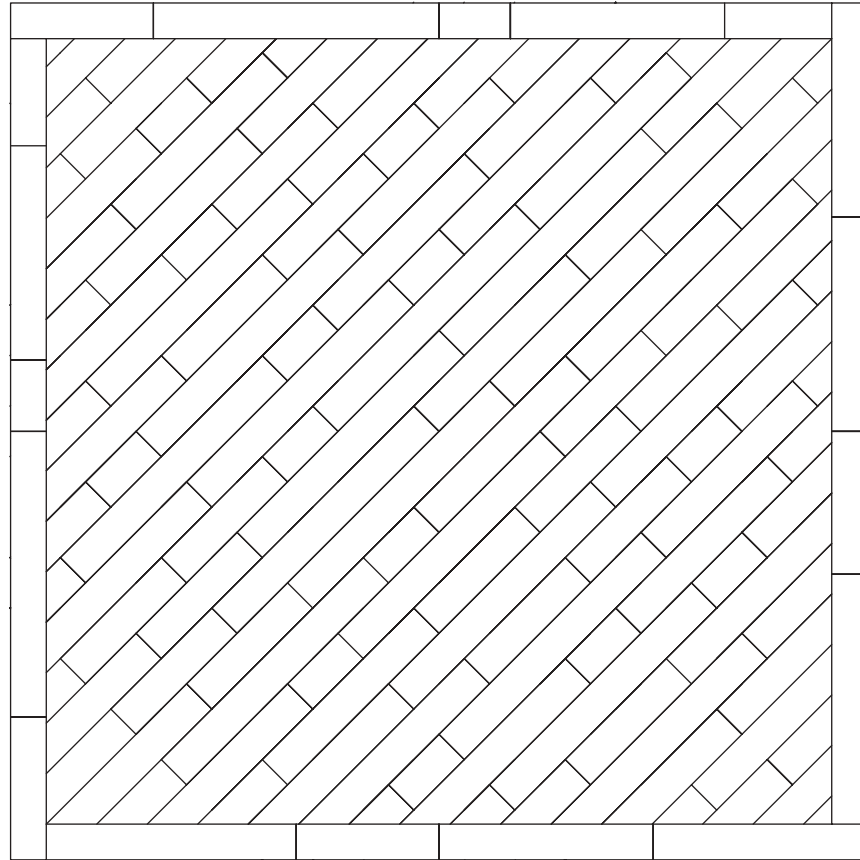
PATTERN #4 6" RANDOM LAYOUT 12' X 12' AREA SHOWN 144 sq. ft. = 29 Units of Planking
