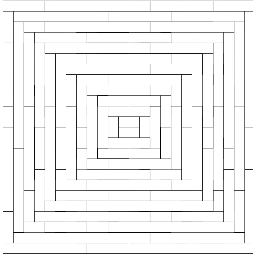
PATTERN #6 6" RANDOM LAYOUT 12' X 12' AREA SHOWN 144 sq. ft. = 29 Units of Planking
