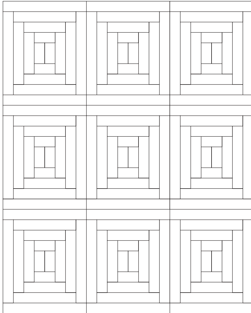
PATTERN #1 6" LAYOUT 12' X 15' AREA SHOWN 180 sq. ft. = 36 Units of Planking
